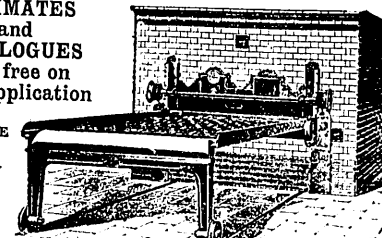
BAKER'S "NEW PATENT DRAW-PLATE" CONTINUOUS BAKING OVEN.
