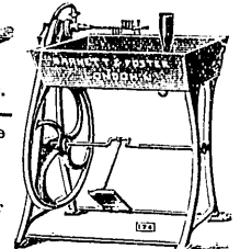
Corking Machine for Beer and Wines.
