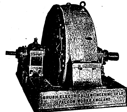
INDUCTOR ALTERNATOR. (MORDEY'S PATENT.)
