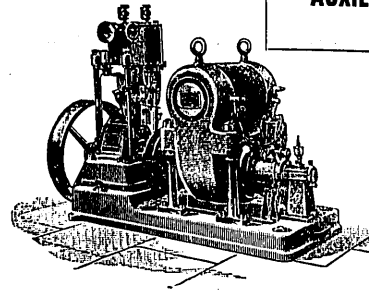
COMBINED ENGINE AND DYNAMO.
