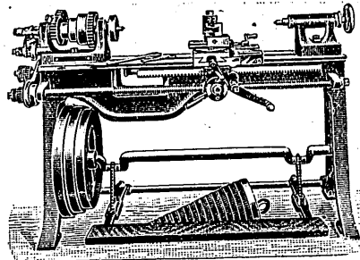
TREADLE LATHES.
