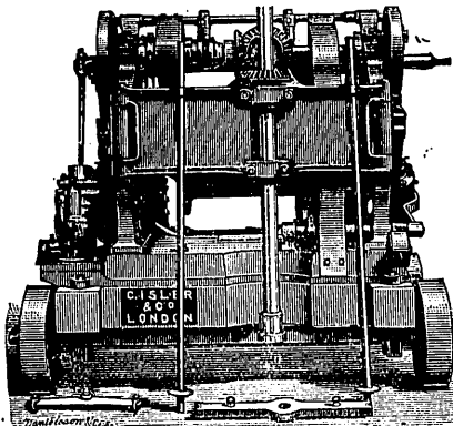
C. ISLER & CO.'S IMPROVED COMBINED CROWN DIAMOND ROCK AND PERCUSSION MACHINERY.
