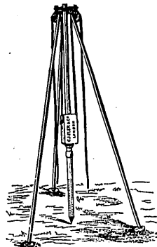
C. ISLER & CO.'S IMPROVED TUBE WELL & DRIVING APPARATUS AS USED IN ALL CAMPAIGNS BY H.M. WAR OFFICE.
