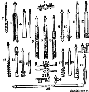
C. ISLER & CO.'S IMPROVED BORING TOOLS FOR WELLS AND FOR PROSPECTING PURPOSES.
